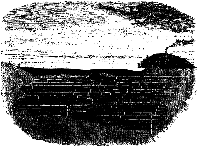
Fig. 150. Section of Tamar Lead Silver Mine, Beerferrers, Devon. A. Inclined plane, leading to workings and underground shaft. B. Entrance to inclined plane. C. The "Spurgin" shaft. D. The flue of the underground engine, two miles long. X. Slides in the ore.
